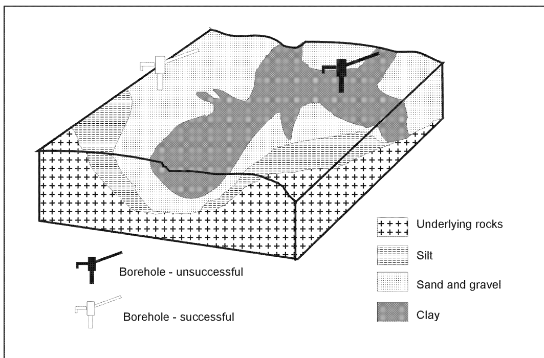
Figure 2.6 Groundwater occurrence in unconsolidated sedimentary rocks.
