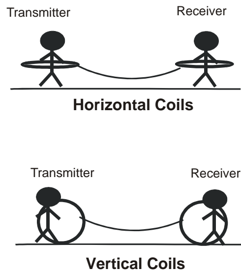
Figure 4.5 The different possible orientations of FEM equipment.
