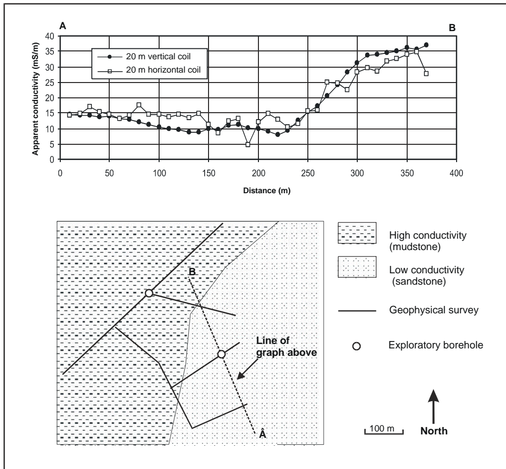
Figure 4.16 Using ground conductivity to map out the boundary between a sandstone and a mudstone in a village.
