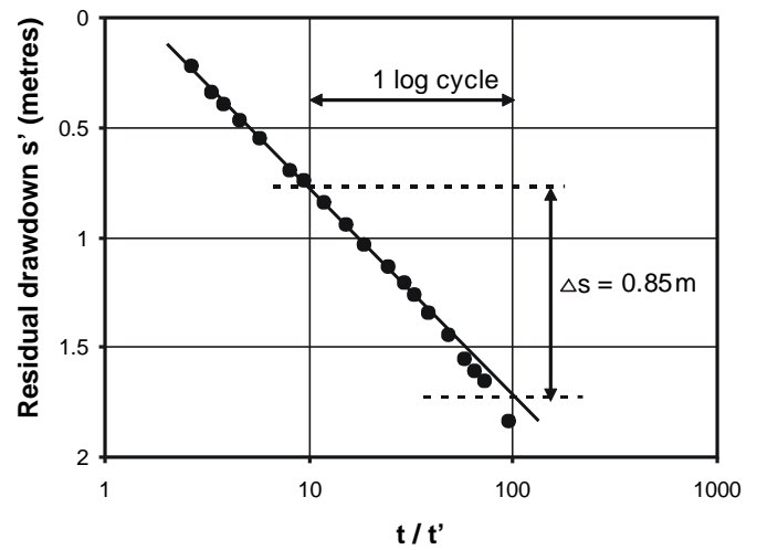
Figure 6.6 An example of measuring \Delta s' from recovery data.
