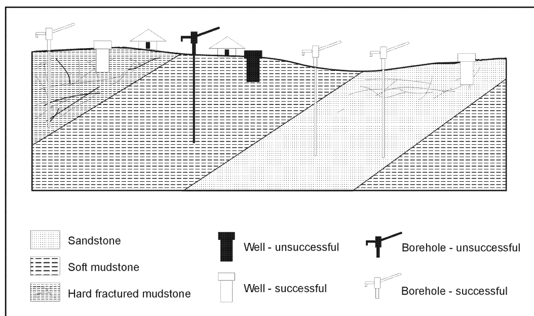
Figure 2.5 Groundwater occurrence in consolidated sedimentary rocks.
