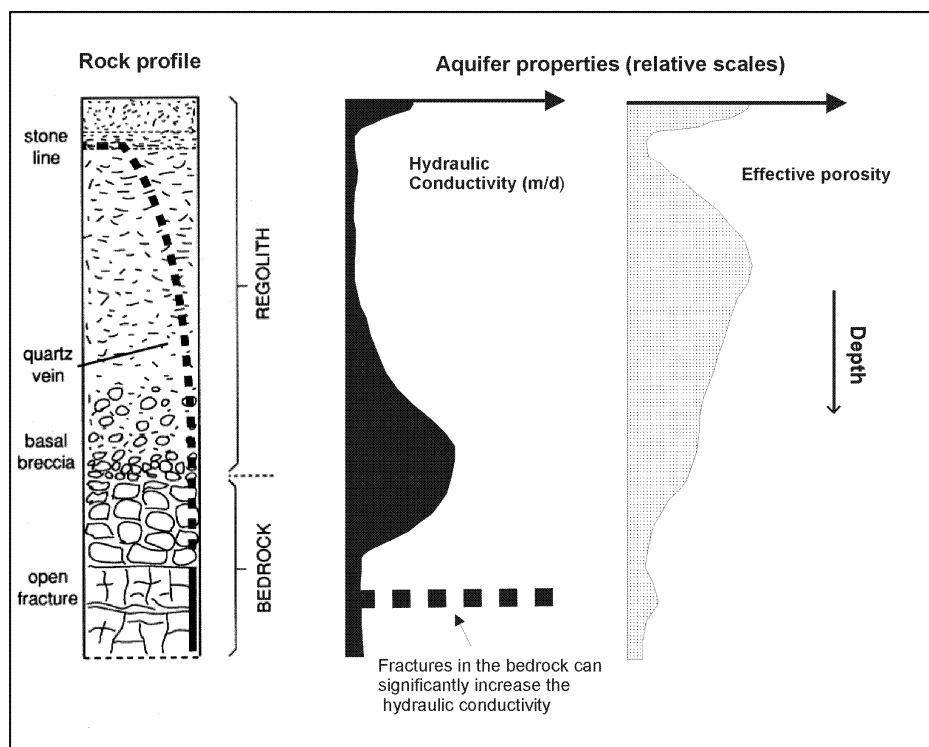
Figure 2.3 Variation of permeability and porosity with depth in basement aquifers (based on Chilton & Foster, 1995).
