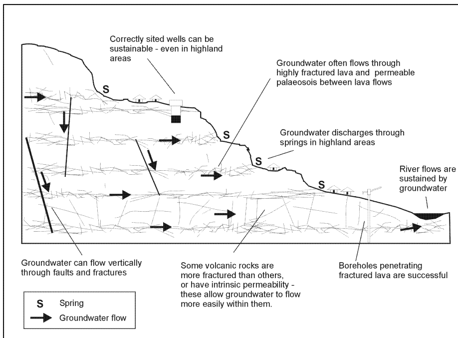
Figure 2.4 Cross section of groundwater flow in highland volcanic areas.
