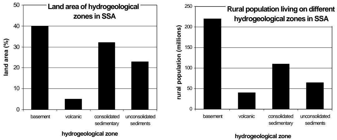
Figure 2.2 Land area and rural population of the different hydrogeological zones of SSA.
