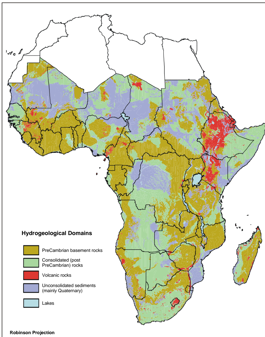
Figure 2.1 Groundwater provinces in sub-Saharan Africa.
